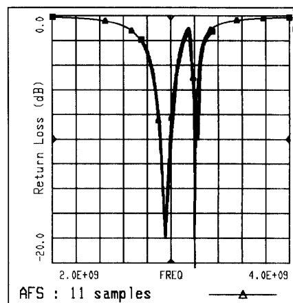
figure 3: Reflection coefficient S11 of patch antenna. —▲— : AFS simulation [2 - 4 GHz] — : reference paper [2.75 - 3.35 GHz]
