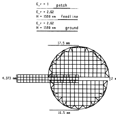
figure 2: Cross section and top view (mesh) of patch antenna.
